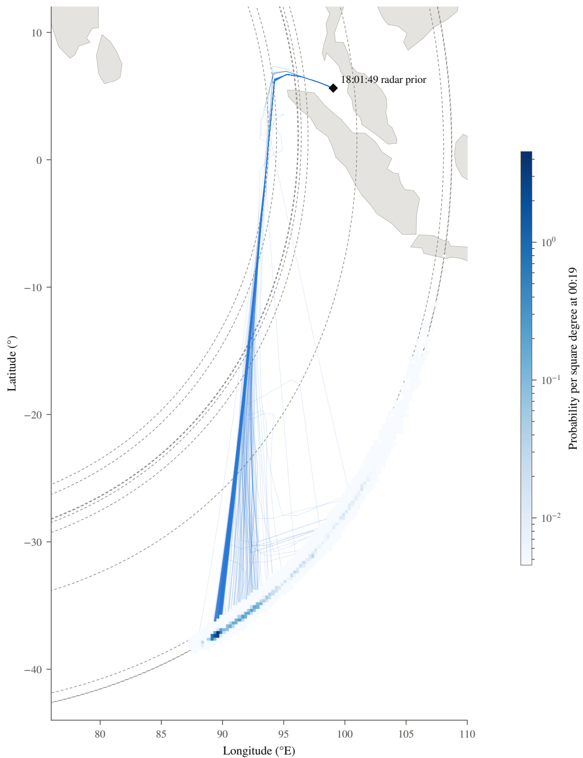
Figure 2. Posterior aircraft position at 00:19 UTC with BTO and BFO, pooled over 4 replicates (blue shading, logarithmic), and 400 routes drawn in proportion to posterior weight from replicate seed 1 (thin lines, 10-minute vertices). Dashed grey curves are the BTO arcs at a reference altitude of 35,000 ft; they are drawn for orientation only. Land: Natural Earth 1:110m.
