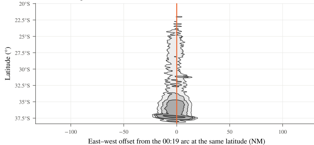
Figure 3. Joint latitude-longitude posterior at 00:19 UTC, drawn as highest-posterior-density regions: the 50% curve bounds the smallest area holding 50% of the probability, and so on outward, so a region here is the smallest place to look for that confidence rather than an interval in either coordinate alone. Binned at 0.05° and smoothed over three bins. Panel a spans the bounding box of the 99% region, so sparse outlying cells are excluded; enclosed areas (NM 2 , at the view's mean latitude) are 99% 17,079, 95% 6,901, 90% 3,859, 50% 330. Panel b replots the same particles against their east-west offset from the 00:19 arc, because the region is about 0.3° wide and 18° long and the inner contours are not separable at a true aspect ratio. Arcs are the reference BTO loci at 35,000 ft; 00:19 is the 7th. Land: Natural Earth 1:110m.
